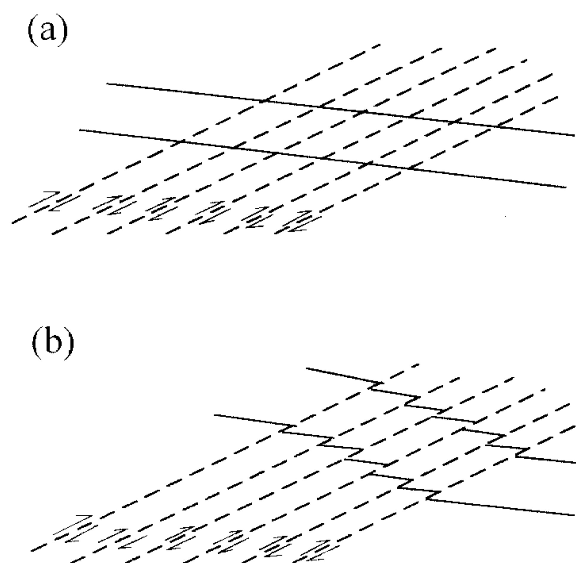
Fig. 7. A sketch showing how the bending of the seismic belt along the fore-arc basin of the Ryukyu arc-trench system is possibly bent by the Central Taiwan NE-SW Fault Zone. (a) seismic belt along the fore-arc basin in the Ryukyu arc-trench system before the bending; (b) the same seismic belt after the bending.
